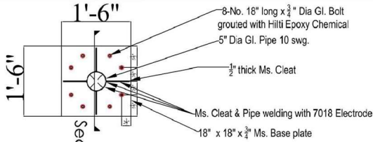
Typ. Detail. Base Plate
