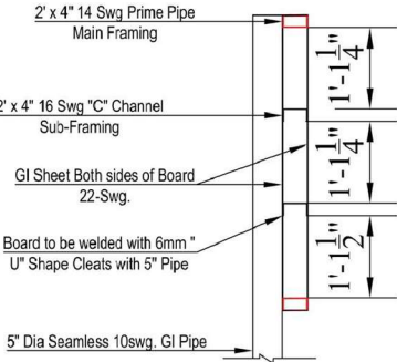
Section 1-1
