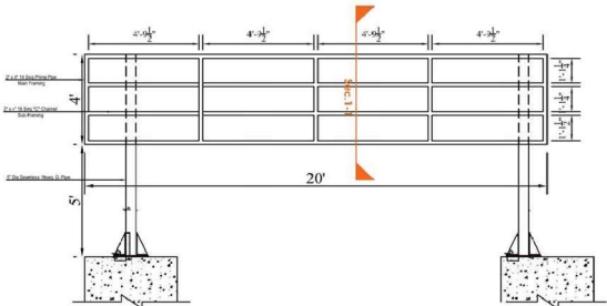
Board Front Elevation
