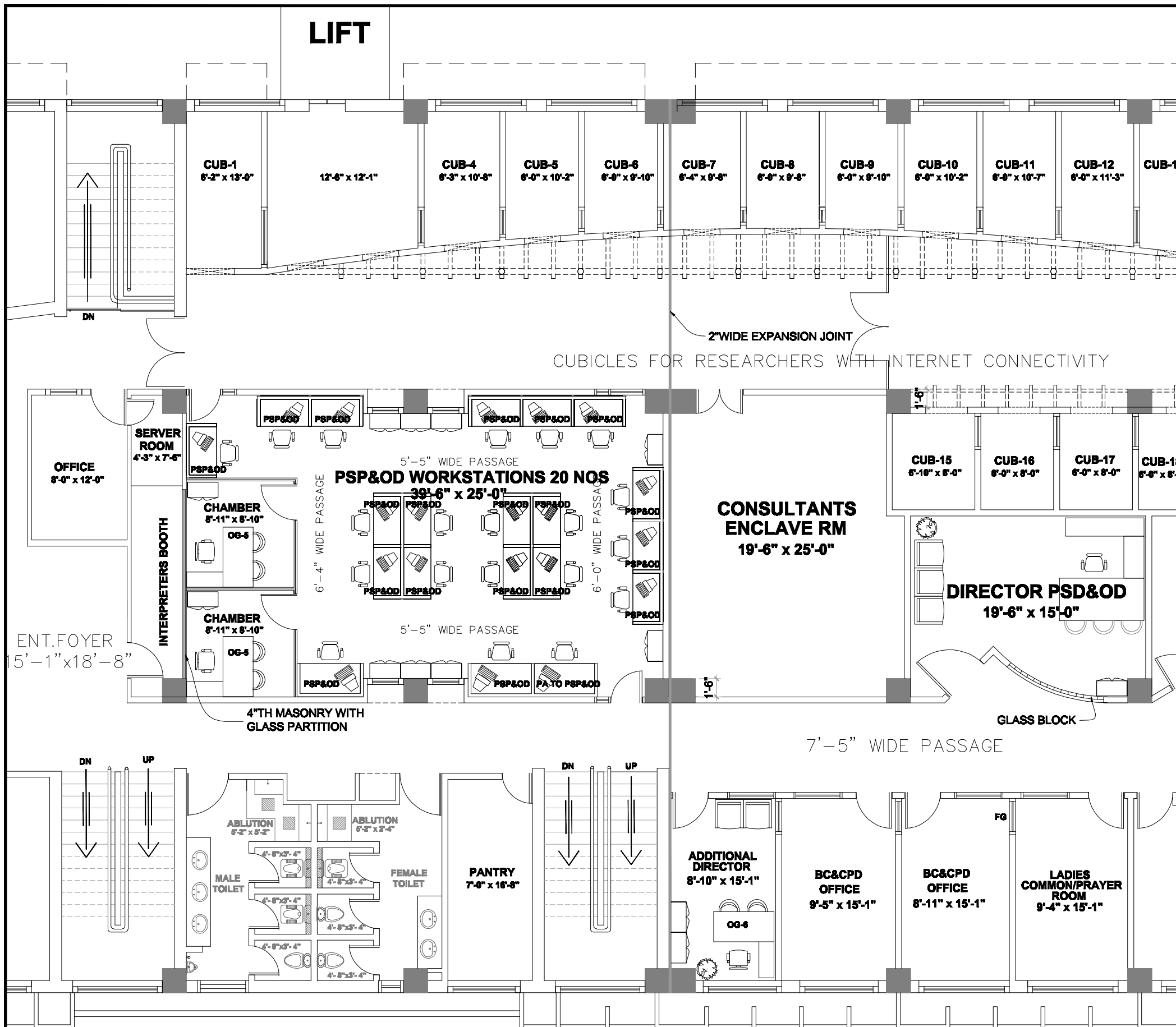
PART PLAN OF PROPOSED PSP&OD AT 2nd FLOOR LRC BUILDING
