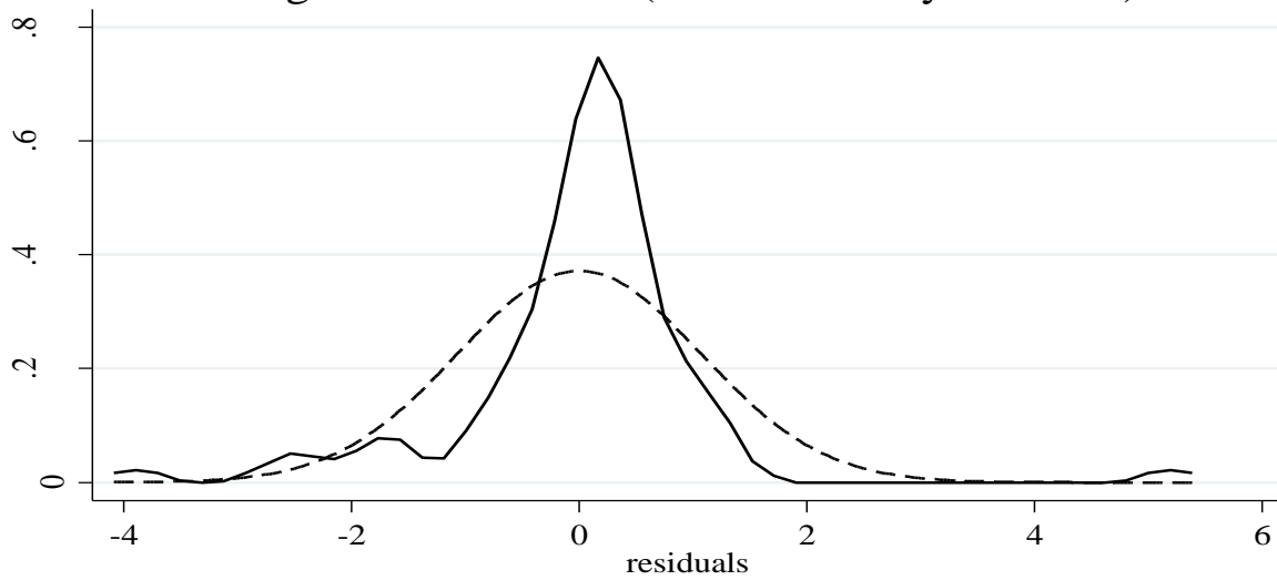
Figure A5: Model 5 (Kernel Density Estimate)
