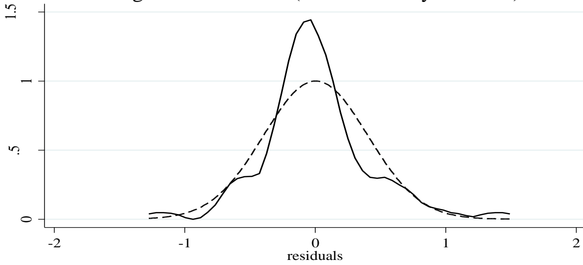
Figure A4: Model 4 (Kernel Density Estimate)
