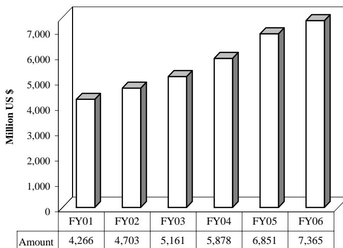
Figure 1: Export Receipts
