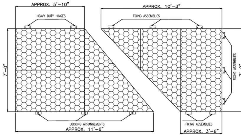
TYPE-2 PANEL
