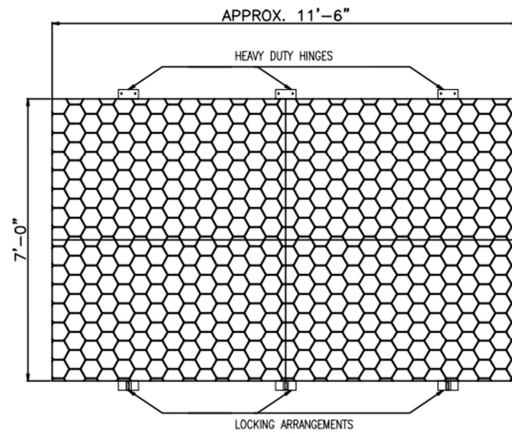
TYPE-1 PANEL
